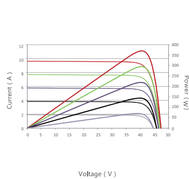
Current-Voltage & Power-Voltage Curves (360W)
